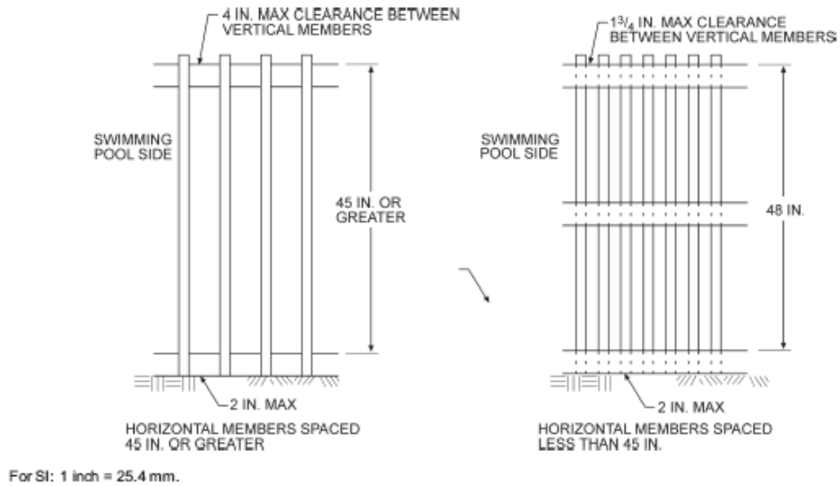
Figure AG105.2(2) PRIVATE SWIMMING POOL BARRIER CONSTRUCTION
